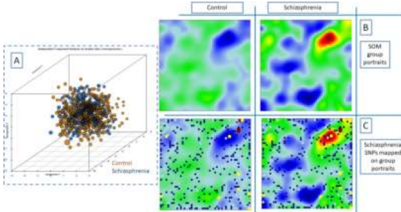
Figure 2. PCA plot and SOM portraits of schizophrenia cases and controls. A) PCA plot for schizophrenia and controls B) SOM group portraits of schizophrenia and control samples. C) Schizophrenia-associated SNPs displayed on the group portraits, dot sizes, and colors indicate the number of SNPs in the metagene (as the size increases and the color changes from blue to red, the number of SNPs increases)
