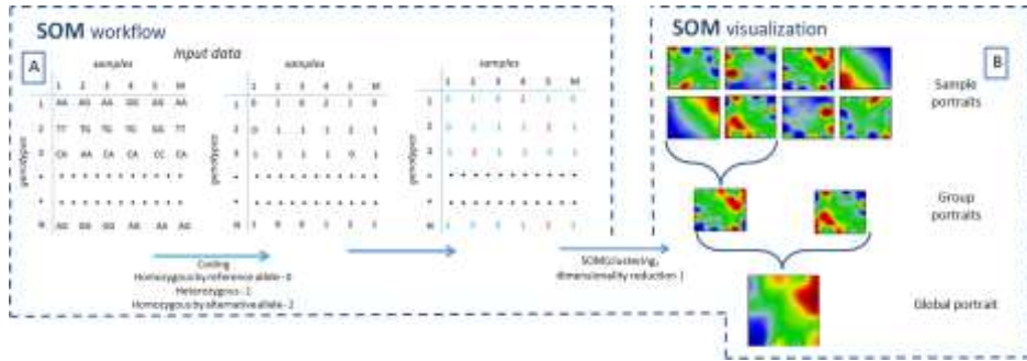
Figure 1. SOM pipeline. A) The genotypes were transformed to a numeric matrix, then the SOM algorithm reduces the dimensionality of input data, simultaneously clustering samples with similar genotypes. B) At the metadata level, it generates individual SOM portraits for each sample, which are then combined in group portraits and in the end the global SOM portraits.
