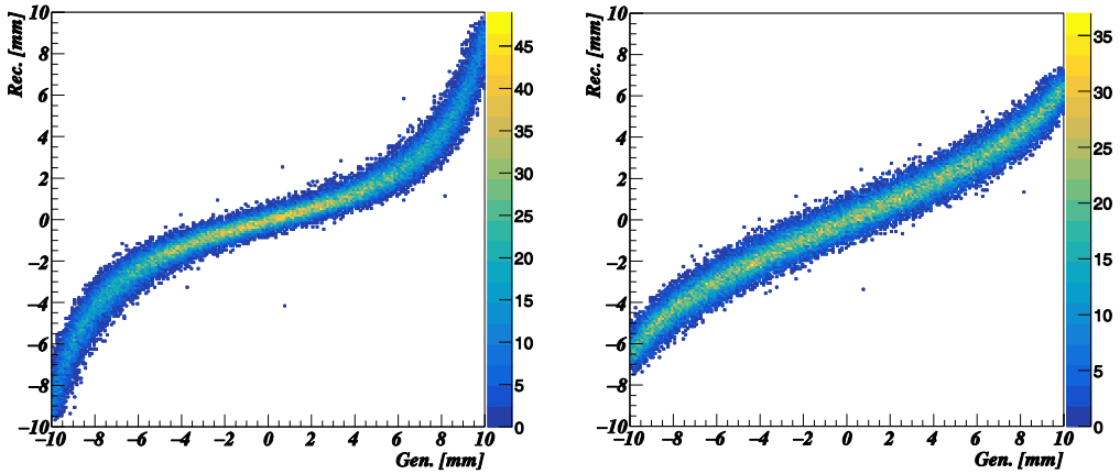
Figure 1. Correlation between reconstructed and generated x positions of the incident electrons for the case \omega_i = E_i (left plot) and \omega_i = \sqrt{E_i} (on the right).
