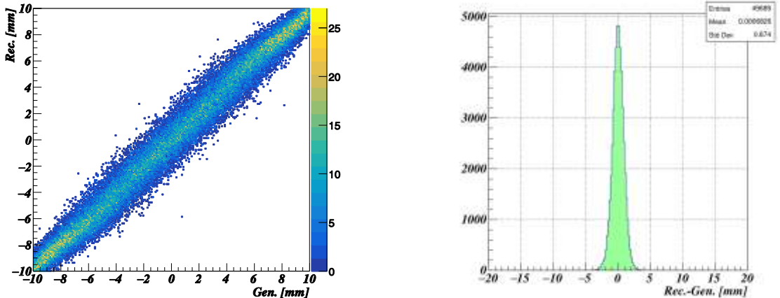
Figure 3. Correlation between X_{rec.} and X_{gen.} (left) and their difference (right) for logarithmic weighting and a cutoff parameter W_0 = 3.6 .
