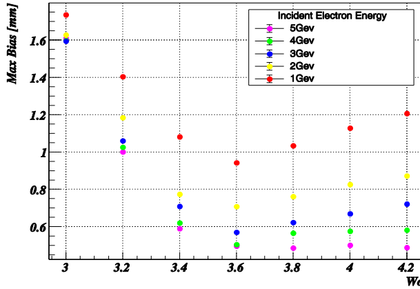
Figure 2. Dependence of maximum bias on cutoff parameter W_0 for incident electron energies of 1–5 GeV.
